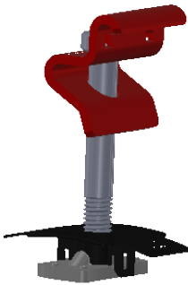
End Clamp Set
